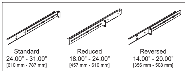
Rear Bracket Settings
