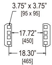
Mounting Dimension (Square Rails)
