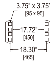
Mounting Dimension
