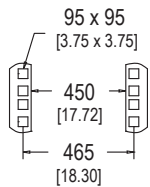
Mounting Dimension
